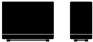
64256 Back – Short with Kick Protect Border Height 28.0” Width 36.5” Depth 15.75”
