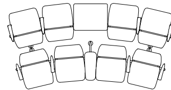
Curved Unit Back to Back with Table 117.0"Lx62.5"Dx33"H - 2971 mm x 1587 mm x 838 mm
