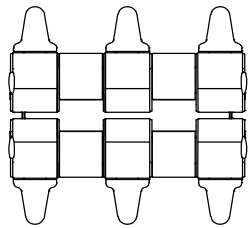
6 Seat Unit Back to Back with Footrest and Intermediate Tables
